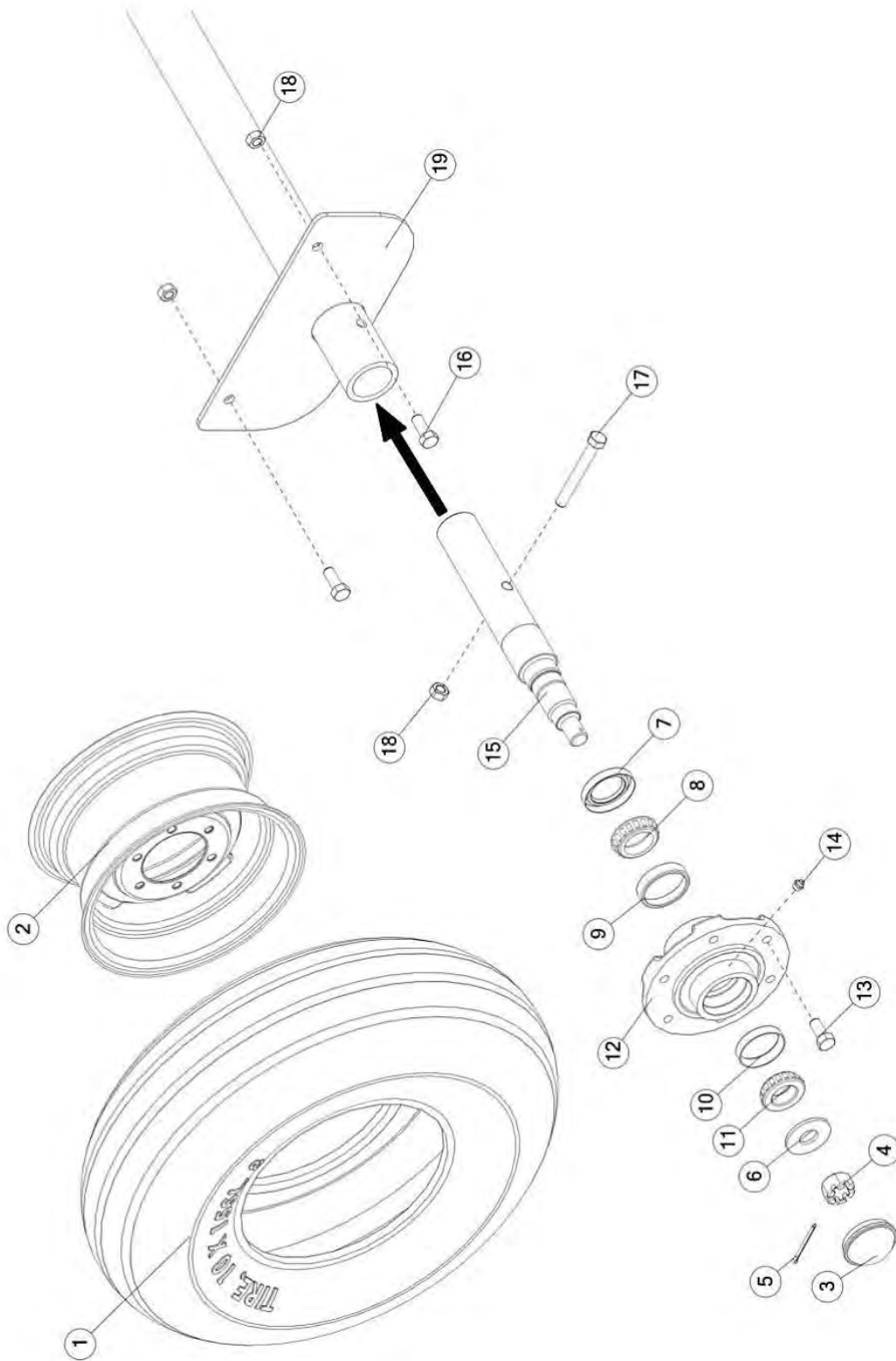
FIGURE 14 HUB ASSEMBLY
